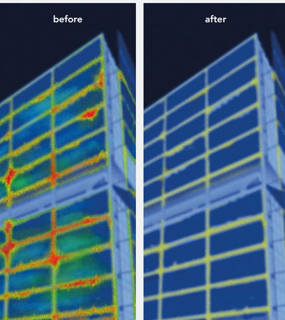
Heat loss image of a building before and after proper window sealing.
